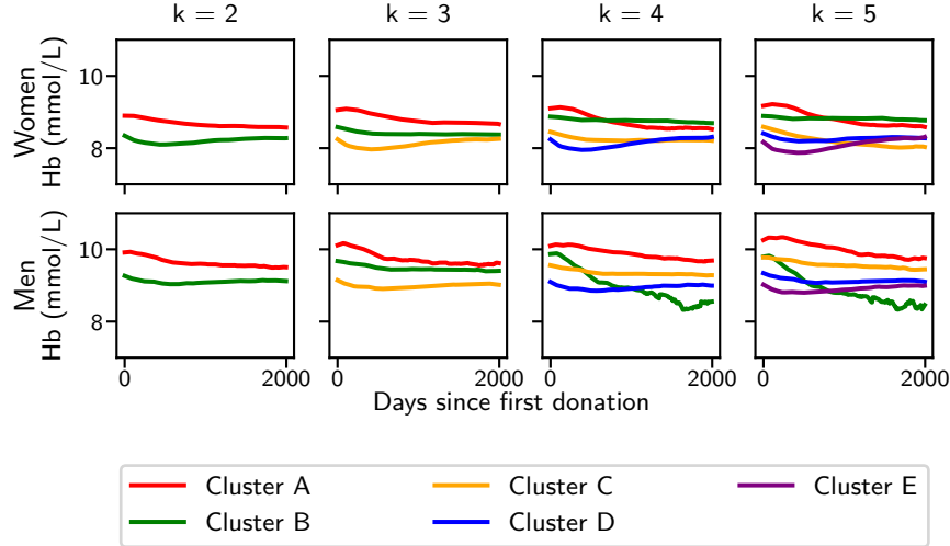
Fig. 3. Cluster centroids after clustering resampled Hb trajectories of 5000 female and 5000 male donors based on the intercept and slope of the linear trend, using the k -means clustering algorithm ( k = \{2, 3, 4, 5\} ). The limits on the y-axis are equal to those of Figure 2 for comparison.
