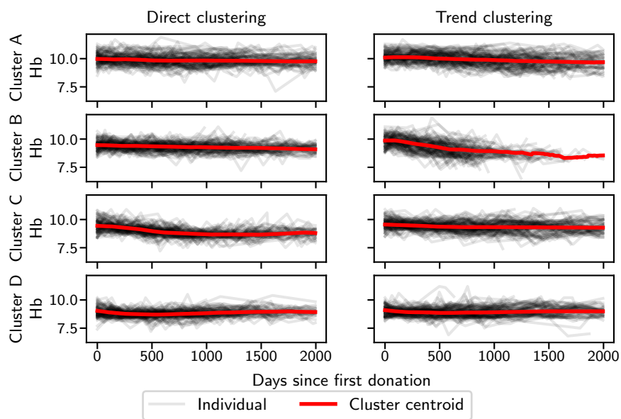
Fig. 4. Cluster centroids after clustering resampled Hb trajectories of 5000 male donors, using direct (left) or trend clustering (right) and k-means clustering with k = 4 . Red lines are the cluster centroids. 100 randomly sampled individual Hb trajectories from each cluster are also plotted to show the fit.
