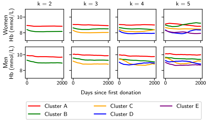
Fig. 2. Cluster centroids after clustering resampled Hb trajectories of 5000 female and 5000 male donors with the k-means clustering algorithm ( k = \{2, 3, 4, 5\} ) and DTW distance as distance measure.
